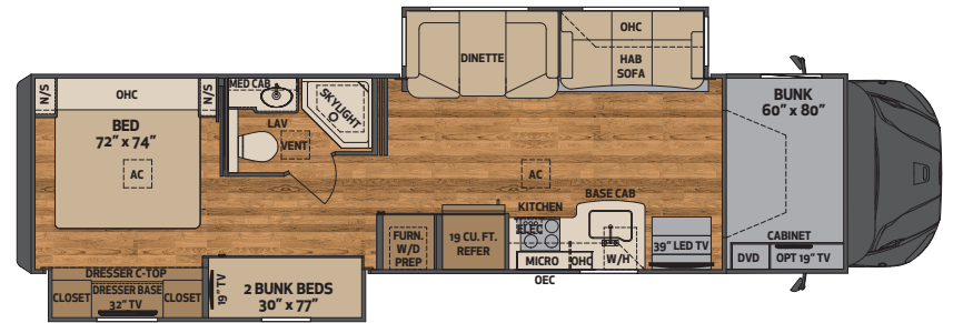
Wheelbase 279"
