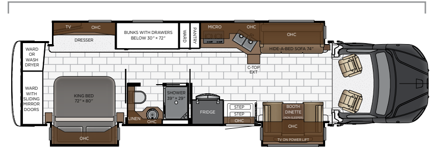
Length: 40' 11"
