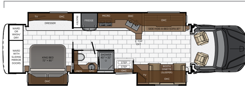
Length: 40' 11"
